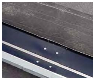
Refit the overlapping water locks together with a hand seamer.
